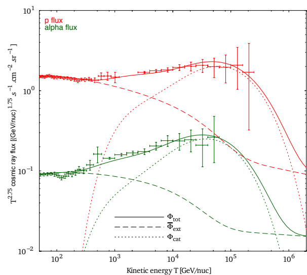
Figure 1: Proton (upper curve) and helium (lower curve) spectra in the range extending from 50 GeV/nuc to 100 TeV/nuc, for the propagation parameters of model A (see Table 1), giving the best fit to the PAMELA [4] and CREAM [2] data : supernovae explosion rate v = 0.8 century -1 . Solid lines show the total flux, short-dashed lines show the flux due to the sources of the catalog, and the long-dashed curve the flux due to the rest of the sources.
