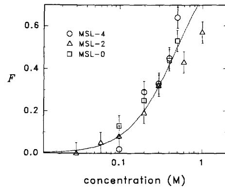
Fig. 3. Plot showing the dependence of the fraction F on the concentration of butanol. F is the fraction of the mobile component which becomes restricted after butanol treatment and it is obtained, as indicated in the text, from the spectral analysis of the EPR profiles of the \text{Ca}^{2+} -ATPase labeled with MSL. The solid curve is an aid to the eyes.
