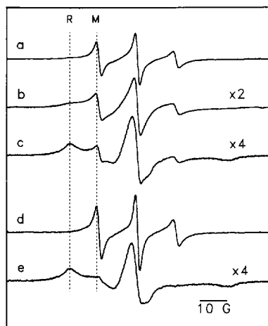
Fig. 1. EPR spectra of maleimide spin-labeled Ca^{2+} -TPase of SRV. (a): MSL-4, (b): MSL-2, (c): MSL-0, (d): difference spectrum obtained as [(a) - 0.375(c)] representing the mobile component and (e): difference spectrum obtained as [(c) - 0.06(d)] representing the restricted component. R and M indicate the low-field peaks of the restricted and mobile components, respectively. All the spectra are normalized to the same double integral with amplification factors indicated in the figure.
