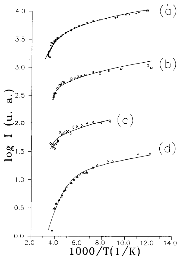
Fig. 2. The temperature dependence of the intensities of EPR spectra of Hb: (a) powdered; (b) R conformation; (c) 75% glycerol; (d) T conformation. The solid lines are examples of the theoretical fits using the values of free energies and entropies given in the text.
