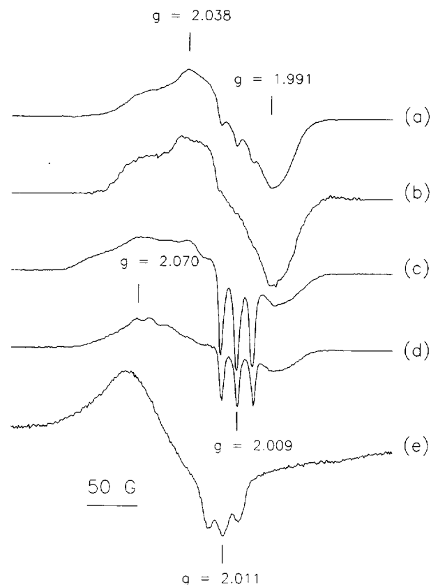
Fig. 1. EPR spectra of different human HbNO samples at 80 K: (a) R conformation; (b) 75% glycerol; (c) T conformation; (d) powdered sample; (e) denatured.
