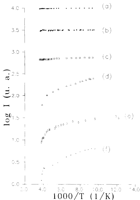
Fig. 3. The temperature dependence of the intensities of EPR spectra: (a) g -marker ( \text{MgCr}^{2+} ); (b) hematin-NO; (c) native MbNO; (d) denatured MbNO; (e) native HbNO; (f) denatured HbNO.
