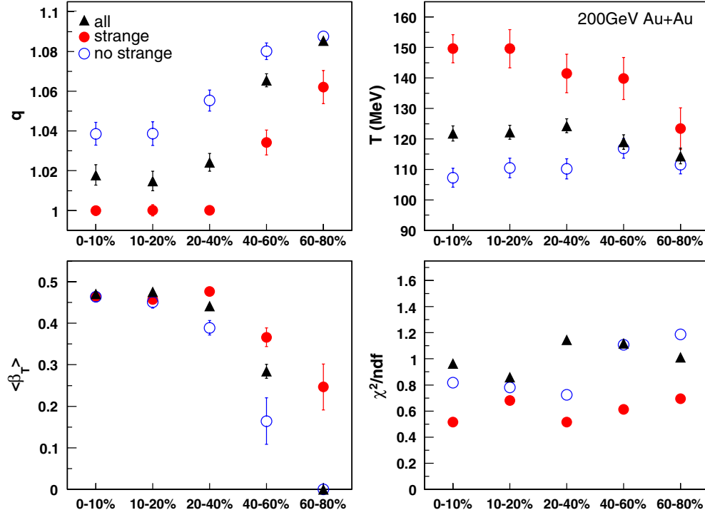
Figure 4. q , T , \beta and \chi^2/\text{nDoF} as a function of centrality for different groups of hadrons from the TBW model fit to spectra in Au+Au collisions at RHIC top energy.
