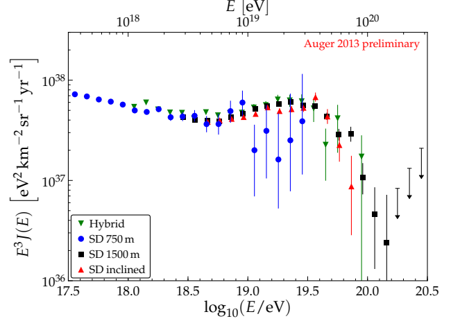
Figure 4: Energy spectra, corrected for energy resolution, derived from SD and from hybrid data.
