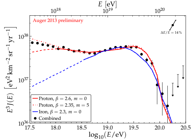
Figure 6: The combined energy spectrum compared to energy spectra from different astrophysical scenarios (see text).
